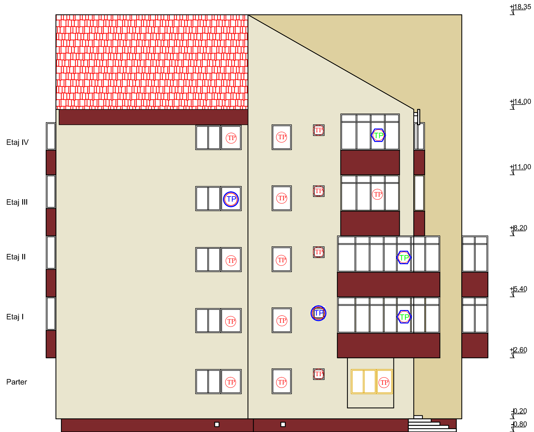
Fatada lateral stanga propusa Scara 1:100
